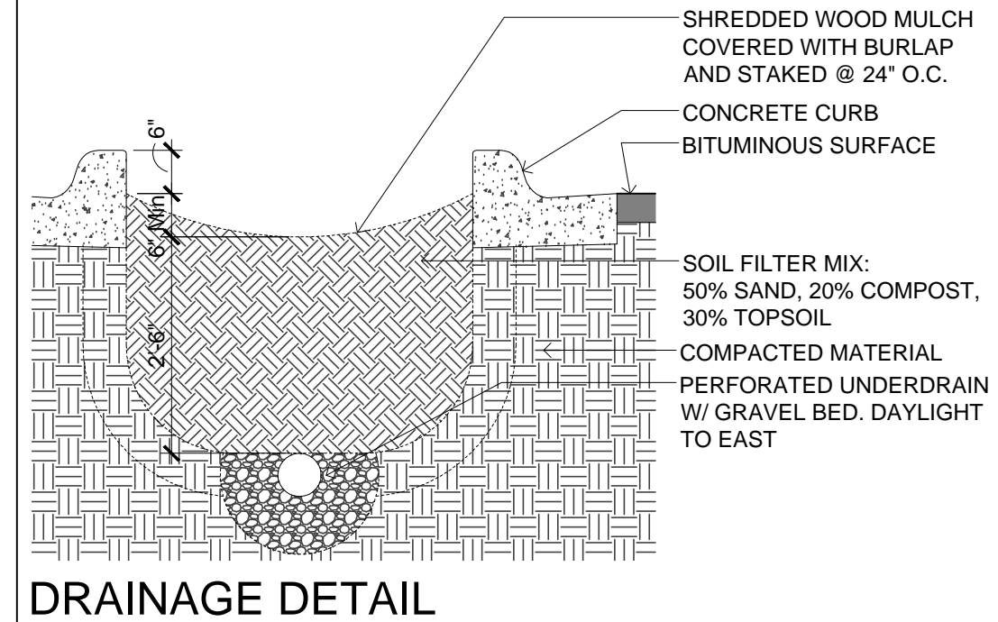
DRAINAGE DETAIL
